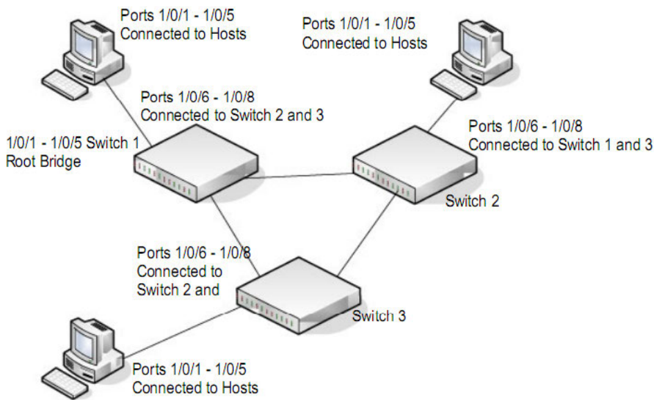
Figure 4. MSTP example configuration
