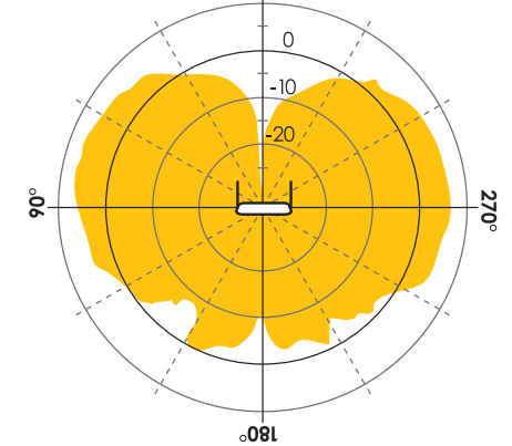
5 Ghz Vertical 0° 10dB
