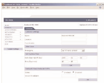
FlexNET GUI
