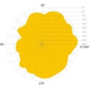
5GHz 2D Radiation Pattern@ Vertical
