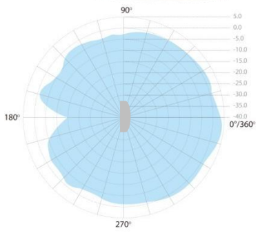
2.4GHz 2D Radiation Pattern@ Vertical
