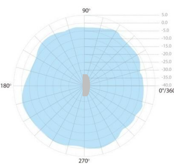
2.4GHz 2D Radiation Pattern@ Horizontal
