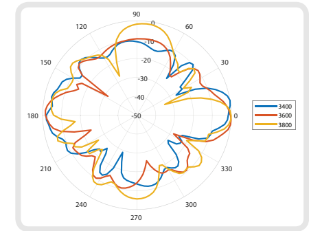
Elevation 2: 3400-3800MHz
