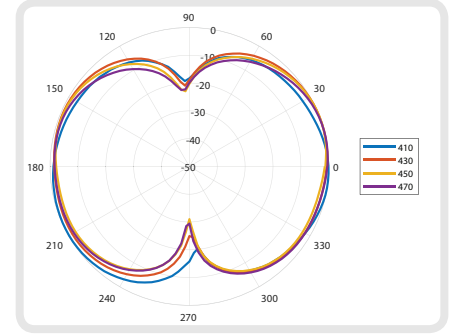
Elevation 1: 410-470 MHz
