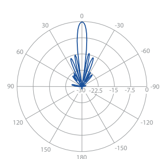
Elevation Pattern H2
