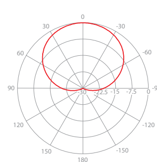
Azimuth Pattern V
