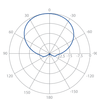
Azimuth Pattern H2
