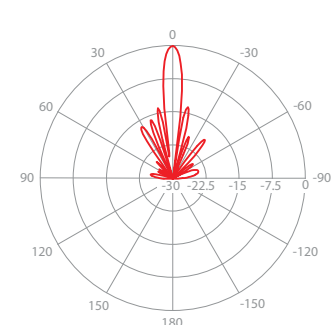
Elevation Pattern V
