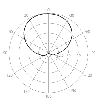
Azimuth Pattern H1
