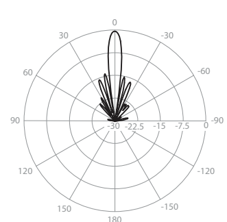
Elevation Pattern H1
