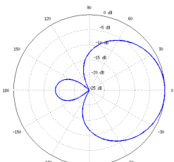
H-Pol Elevation
