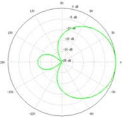
V-Pol Azimuth
