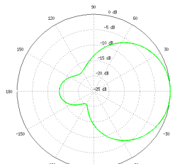
H-Pol Azimuth
